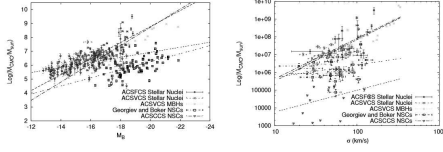
Fig. 1. CMOs masses versus M_B (a), and \sigma of the host galaxies. The black dashed line, black dashed pointed line, black two pointed line, and black pointed line are the least square fit of the Fornax, Virgo, HST/WFCP2, and Coma sample, respectively.
